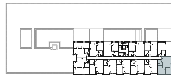
schéma pôdorysu 5.NP / scheme of the fourth floor
