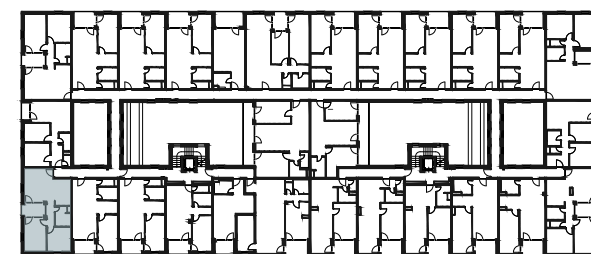
schéma pôdorysu 3. NP / scheme of the second floor
